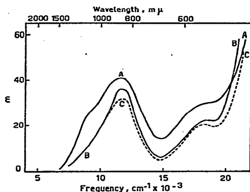
Fig. 3. Absorption and reflectance spectra of [\text{H-sal en NHCH}_3]_2\text{Ni} : A, reflectance spectrum; B, in chloroform; C, in pyridine.
